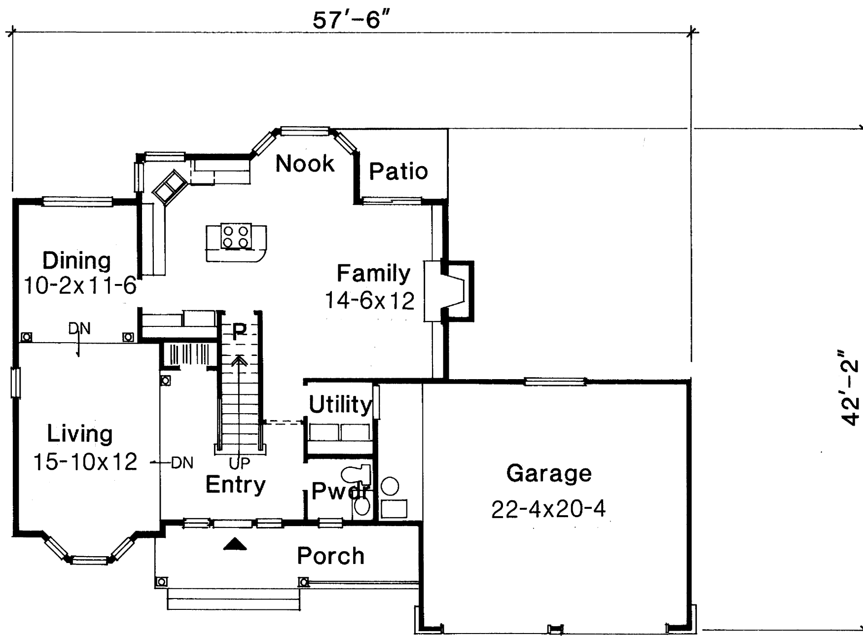
First Floor 1041 Sq. Ft.
