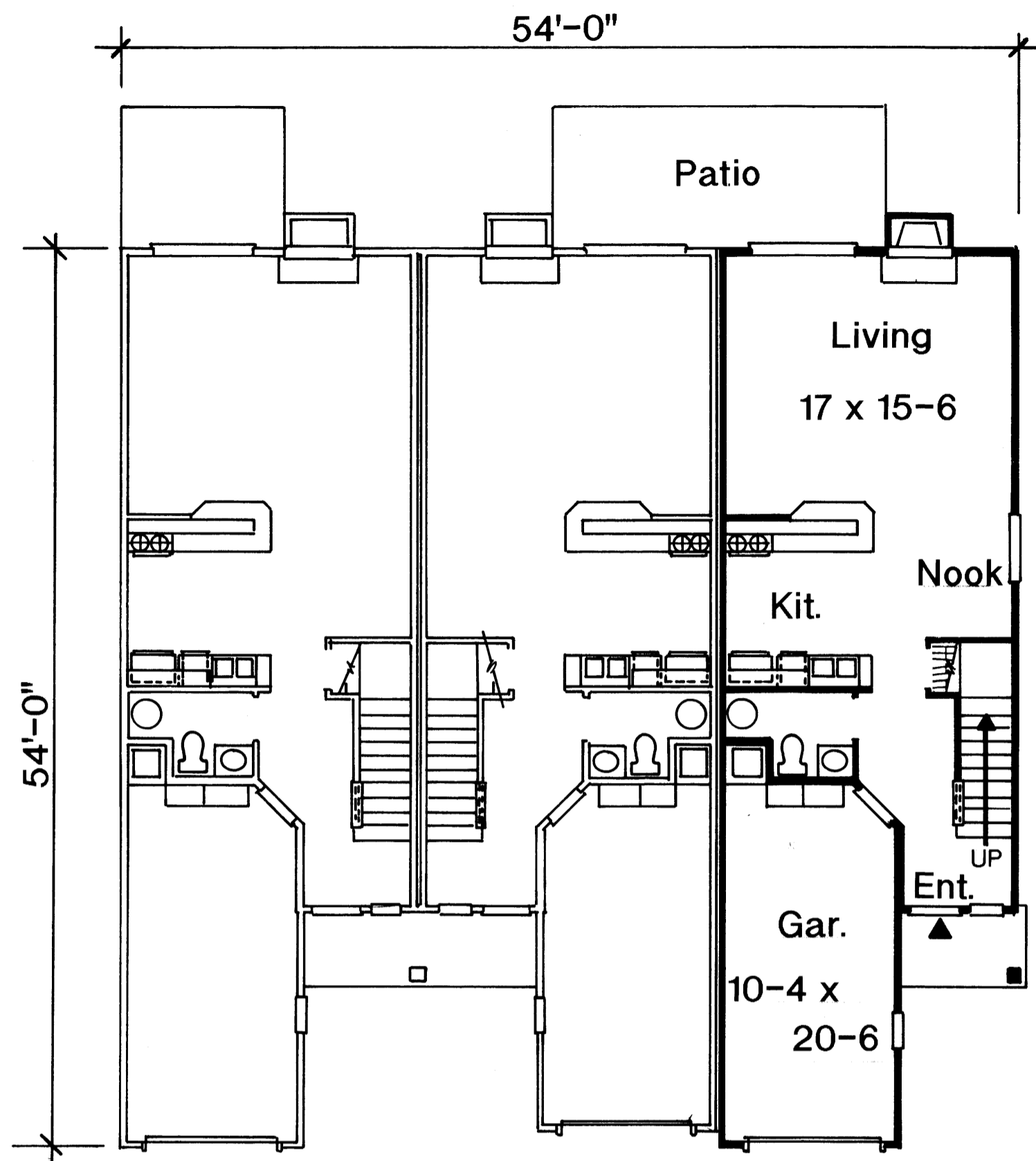
First Floor 637.5 Sq.Ft.
