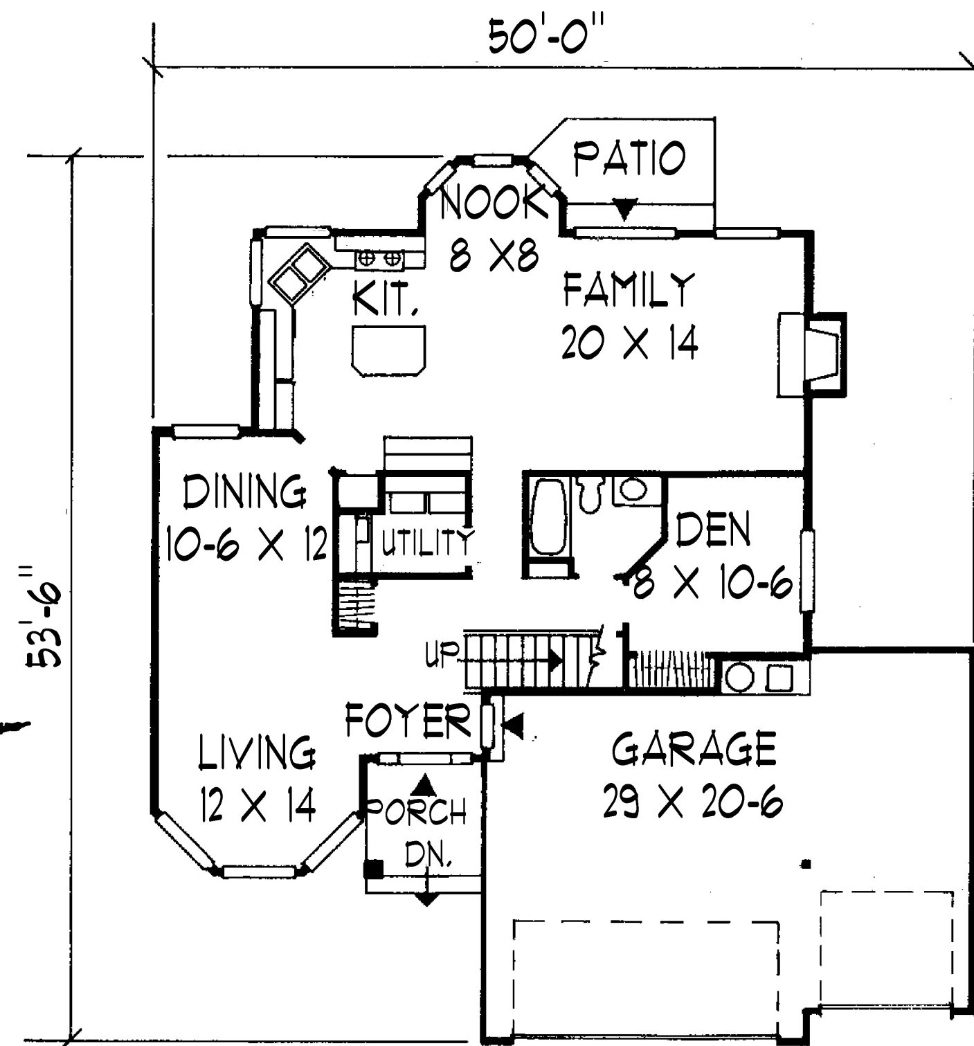
FIRST FLOOR ... 1,128 SQ.FT.
